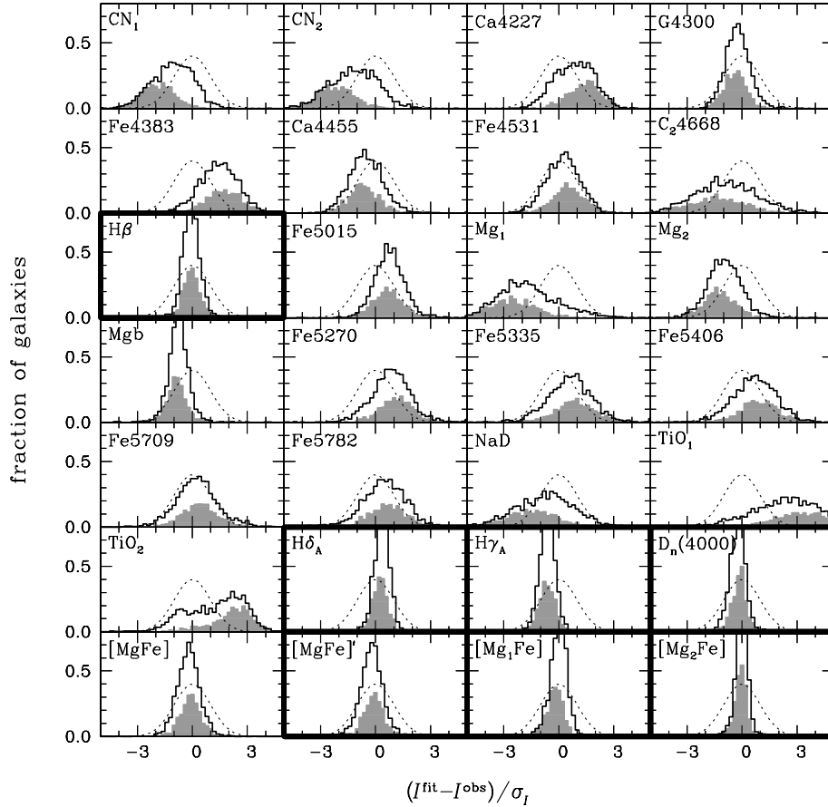
Figure 18. Simultaneous fit of the strengths of several indices in the spectra of 2010 galaxies with S/N_{\text{med}} \geq 30 in the ‘main galaxy sample’ of the SDSS EDR. The highlighted frames indicate the seven indices used to constrain the fits. The stellar velocity dispersion of the models are required to be within 15 \text{ km s}^{-1} of the observed ones. Each panel shows the distribution of the fitted index strength I^{\text{fit}} minus the observed one I^{\text{obs}} , divided by the associated error \sigma_I (equation 3). For reference, a dotted line in each panel indicates a Gaussian distribution with unit standard deviation. The shaded histograms show the contributions to the total distributions by galaxies with \sigma_v > 180 \text{ km s}^{-1} , corresponding roughly to the median stellar velocity dispersion of the sample.
