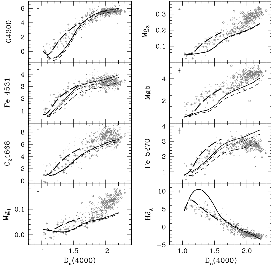
Figure 15. Strengths of G4300, Fe4531, C 2 4668, Mg 1 , Mg 2 , Mgb, Fe5270 and Hδ A as a function of D n (4000) for the same SDSS galaxies as in Fig. 14. The lines show the evolution of the standard SSP model of Section 3 for solar metallicity and for stellar velocity dispersions \sigma_V = 70 \text{ km s}^{-1} (nominal model velocity dispersion, solid line), 150 \text{ km s}^{-1} (dot-and-dashed line) and 300 \text{ km s}^{-1} (dashed line) at ages from 5 \times 10^7 \text{ yr} to 15 Gyr. The long-dashed line shows the evolution of a model with continuous star formation with a law \psi(t) \propto \exp[-t/(4 \text{ Gyr})] , for Z = Z_{\odot} and \sigma_V = 70 \text{ km s}^{-1} .
